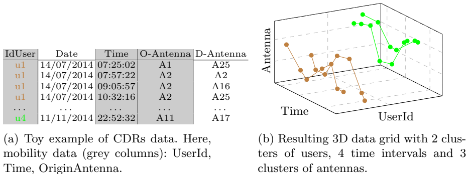
Fig. 1: From 3D mobility data, stemming from CDRs data, to data grid.
