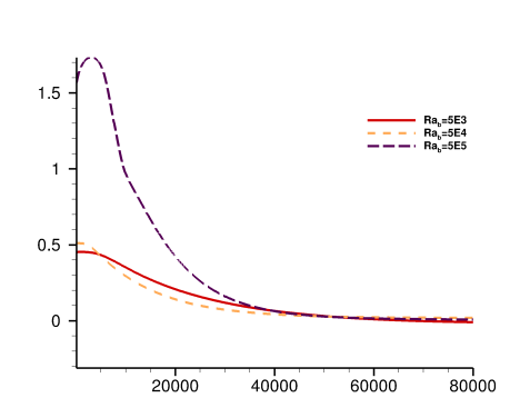
Fig. 13 Evolution of \hat{J} over iteration numbers with Sigmoid-type interpolation functions, for various Ra_b number - Case 4 .
