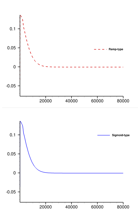
Fig. 12 Evolution of \hat{J} over iteration numbers for Ri = 100 with Ramp-type (top) and sigmoid-type interpolation functions - Case 2 .
