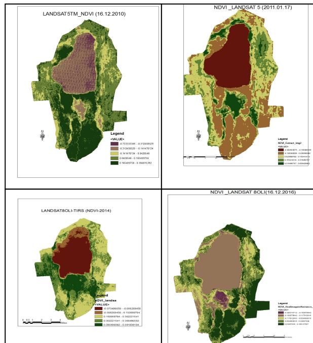
FIGURE 4. NDVI Maps (2010-2016)
