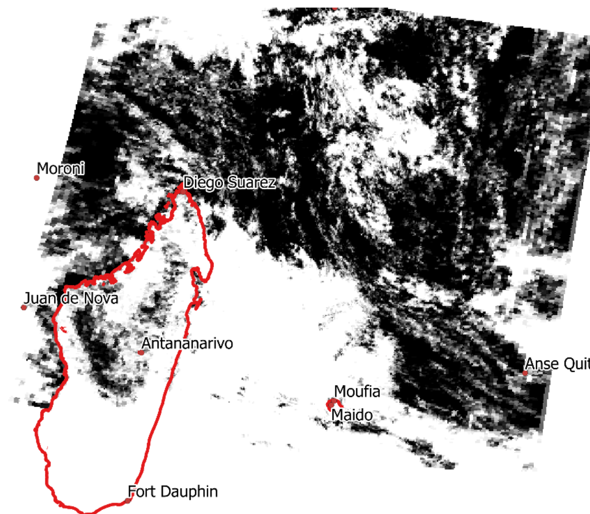
Fig 3: Cloud fraction obtained from Modis
